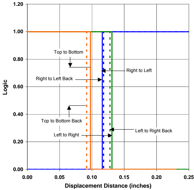
OPB120B - Flag Next to Emitter
